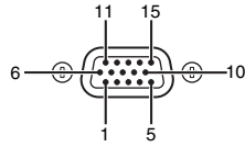
COMPUTER IN/OUT (Mini D-SUB 15-pin)
